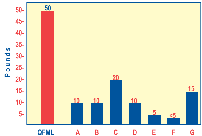
Timken OK Load ASTM D-2509
