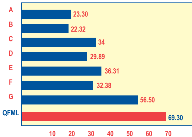
Load Wear Index (LWI) ASTM D-2596
